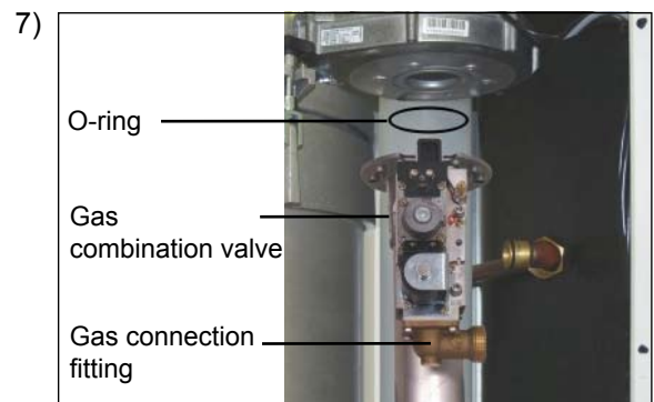
7) Push the O-ring, lubricated with silicone grease, into the packing groove of the fan and fit the mixing chamber with the gas combination valve to the burner fan. Tighten gas connection fitting to gas supply line.
