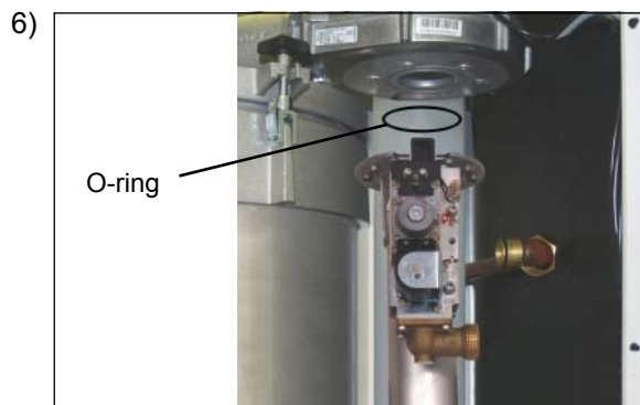
After assembly of the gas restrictor, gas combination valve and air inlet pipe, push the O-ring lubricated with silicone grease into the packing groove of the fan and refit the mixing chamber.
