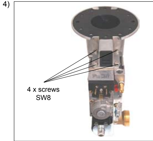
Undo the gas combination valve from the mixing chamber for gas/air (four SW8 screws).
