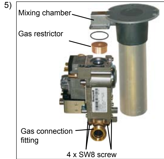
5) Remove the four SW8 screws at the gas connection fitting and remove the fitting from the gas combination valve. Remove the gas combination valve and gas restrictor. Place the protective labels at the valve inlet and valve outlet of the new gas combination valve at the apertures of the removed valve. Return the removed gas combination valve to Wolf.
