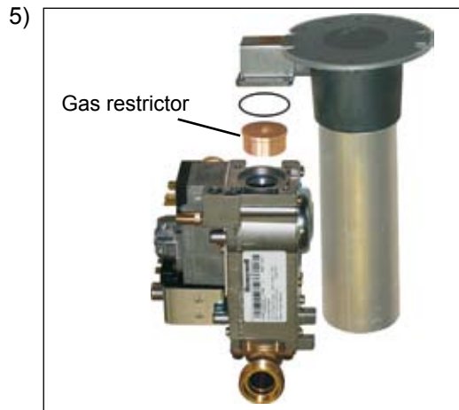
Remove integral gas restrictor and replace with the gas restrictor designed for the new gas type (in accordance with the table on page 66).
