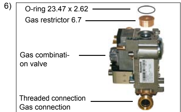
6) Use screws to secure the gas connection fitting with O-ring 26 x 4 to the new LPG gas combination valve (part no. 2744621). Insert new 6.7 gas restrictor (part no. 1730640) into the gas combination valve. Use screws to secure the gas combination valve with O-ring 23.4 x 2.6 to the mixing chamber.
