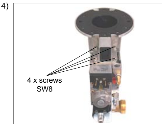
4) Undo the gas combination valve from the mixing chamber for gas/air (four SW8 screws).
